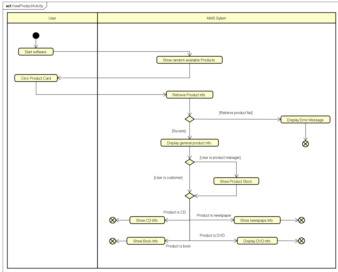
Figure 9: Activity Diagram – View Product
