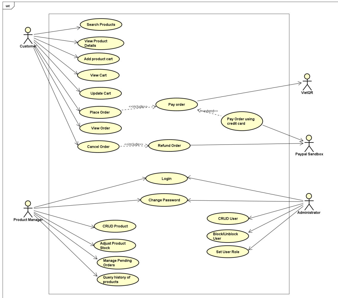
Figure 1: Overall Use Case Diagram
