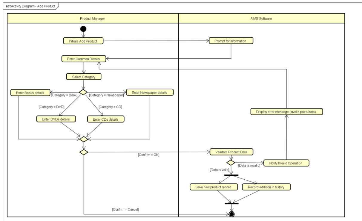
Figure 3: Activity Diagram – Add Product
