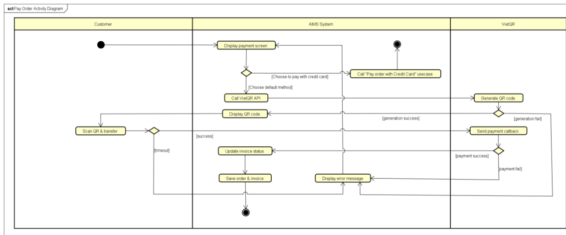
Figure 7: Activity Diagram for Pay Order
