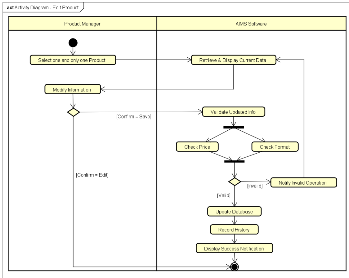
Figure 4: Activity Diagram – Edit Product
