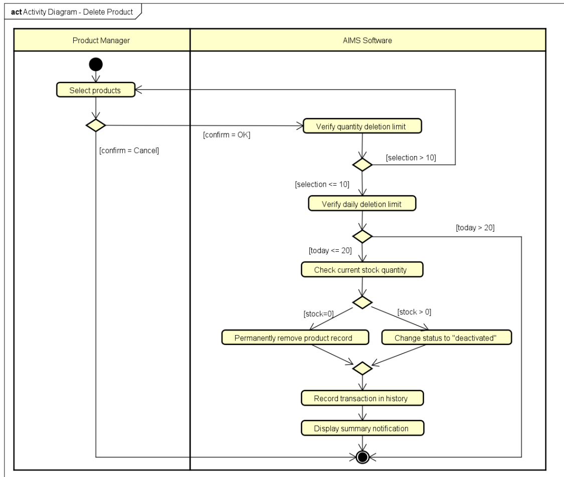
Figure 5: Activity Diagram – Delete Product
