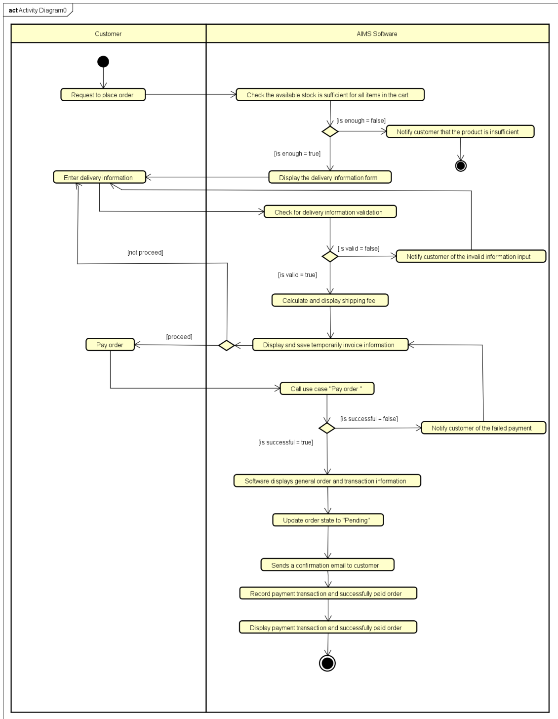
Figure 6: Activity Diagram for Use Case Place Order
